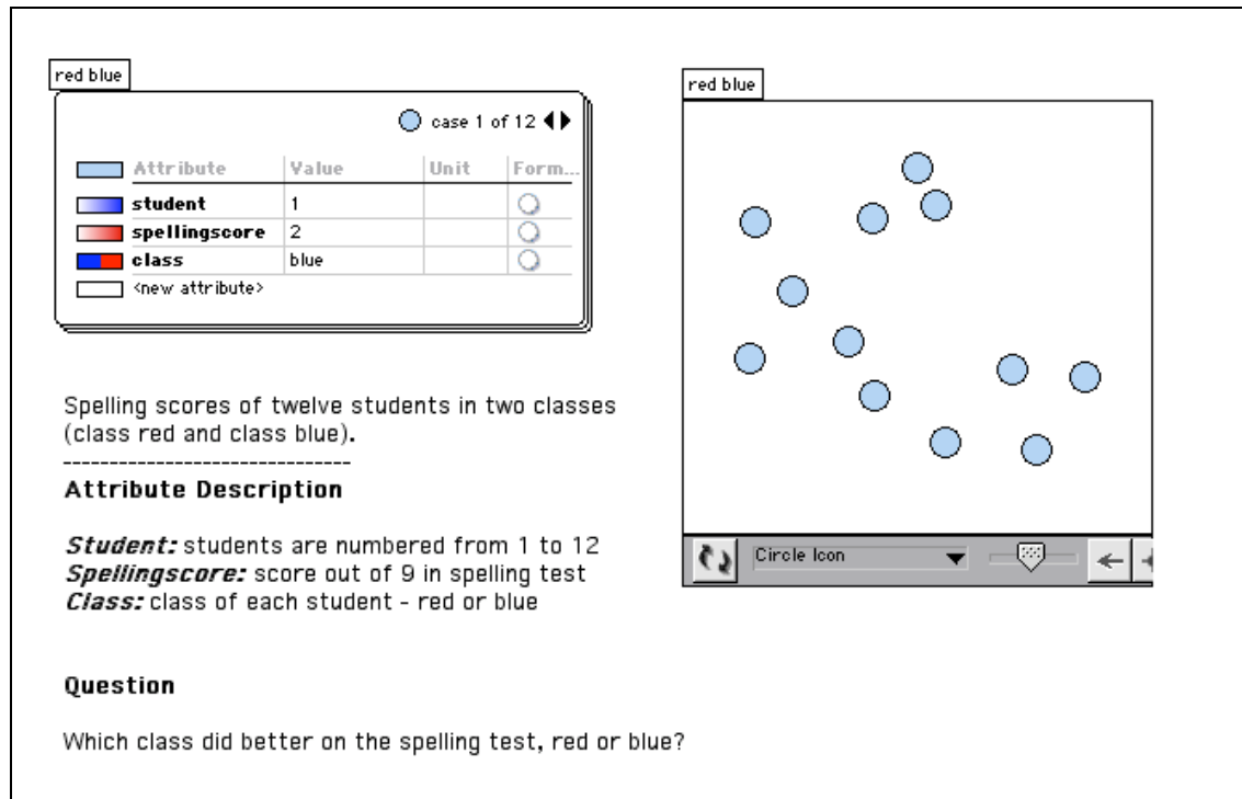
Figure 5: TinkerPlots file for comparing the Red and Blue classes on spelling scores.
