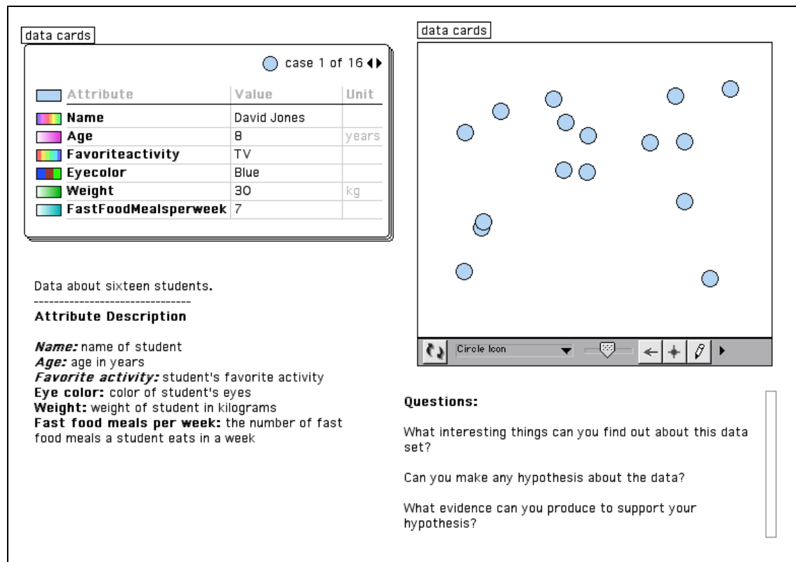
Figure 6: TinkerPlots file for the Data Cards protocol.
